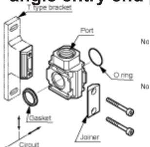
D401-00-(8,10,15)-W-B41W Distributor Block
