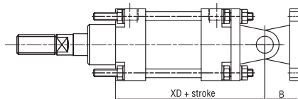
Type AFM Rear Pivot
