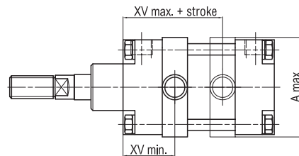
TM Trunion Mount
