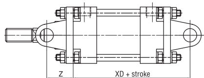
AF Front or Rear Clevis Mount
