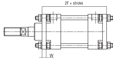
PL Front or Rear Flange Mount
