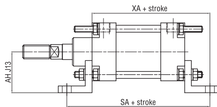
EBN Low Foot Mount
